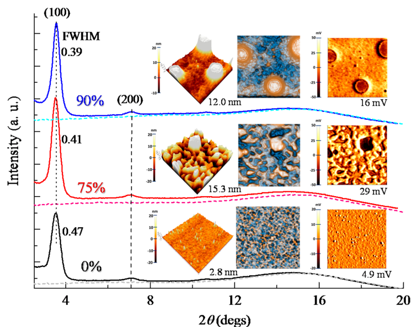
Figure 3. Out-of-plane (solid lines) and in-plane (dashed lines) GIXD spectra of the P3HT:PMMA blending films with different weight percents of PMMA. The fwhm of the (100) peak is also shown. Insets: the corresponding AFM topography (left panels) and phase (middle panels) images and EFM images (right panels). The values of root-mean-square roughness were also indicated on the bottom right corner.
